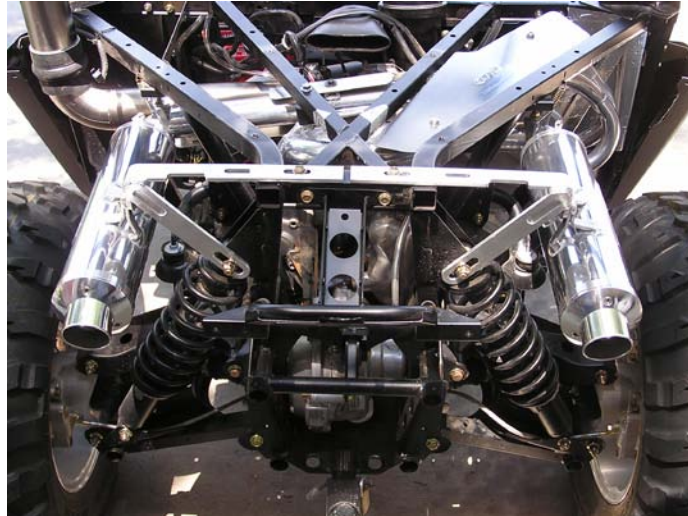
Pic 2 Supplied Bed Heat Shield mounts here
